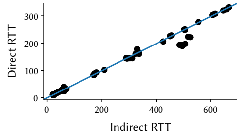
Figure 13: The relationship between direct and indirect round-trip times, \eta , is almost exactly 1/2.
